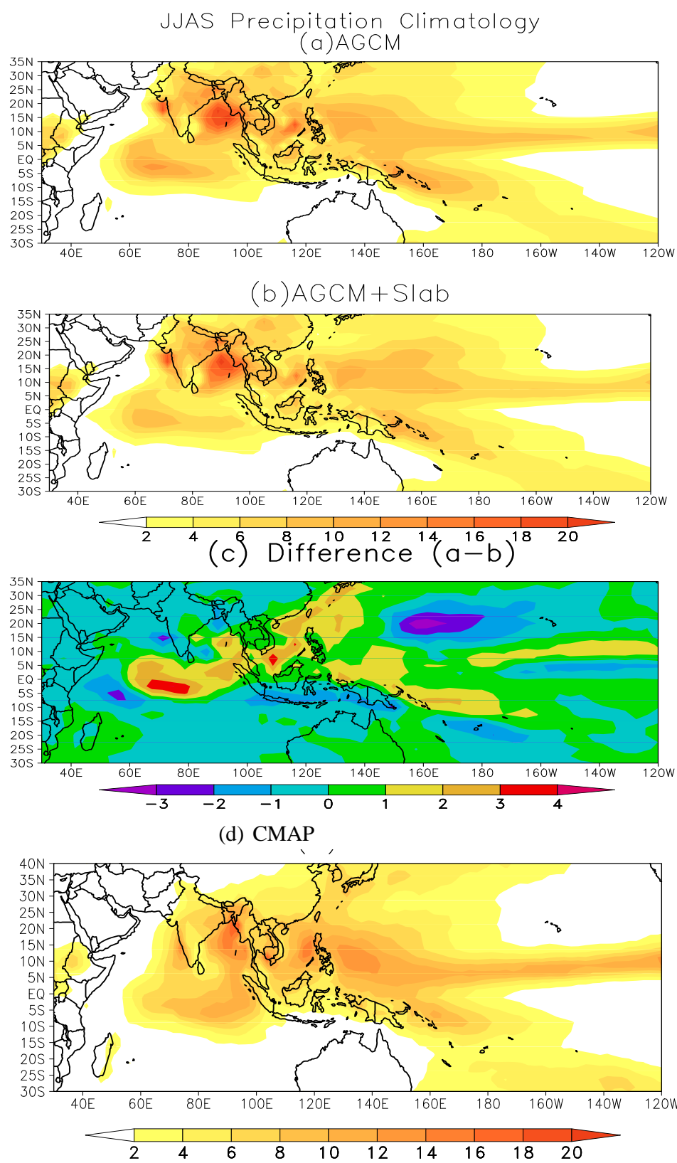
Figure 2. JJAS precipitation ( \text{mm day}^{-1} ) climatology (a) AGCM (b) AGCM+slab ocean model (c) Difference (AGCM-(AGCM+slab)) (d) CMAP
