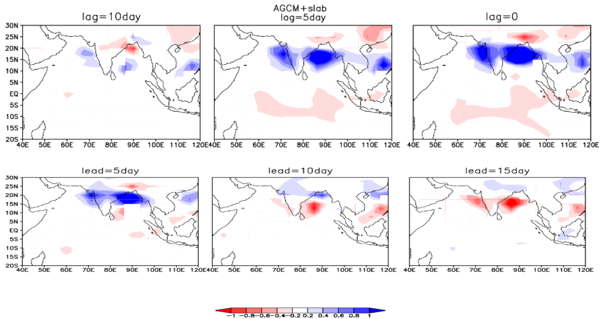
Figure 6. Regressed 20-100 day filtered precipitation (mm day -1 ) anomalies from AGCM for different lags. Only statistically significant (0.1 significance level using t-test) values are plotted.
