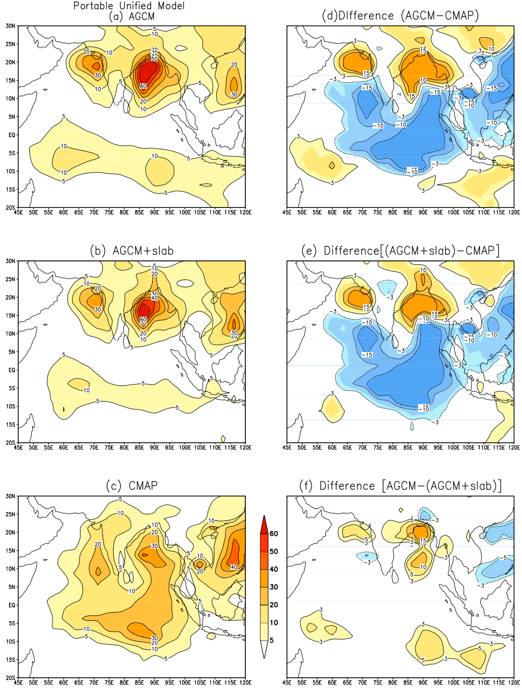
Figure 5: Variance of 20-100 day filtered JJAS precipitation ( \text{mm}^2 \text{ day}^{-2} ) anomalies (1985-1995) (a) AGCM (b) AGCM+slab model (c) CMAP (d) Difference (AGCM-CMAP) (e) Difference ((AGCM+slab)-CMAP) (f) Difference (AGCM-(AGCM+slab))
