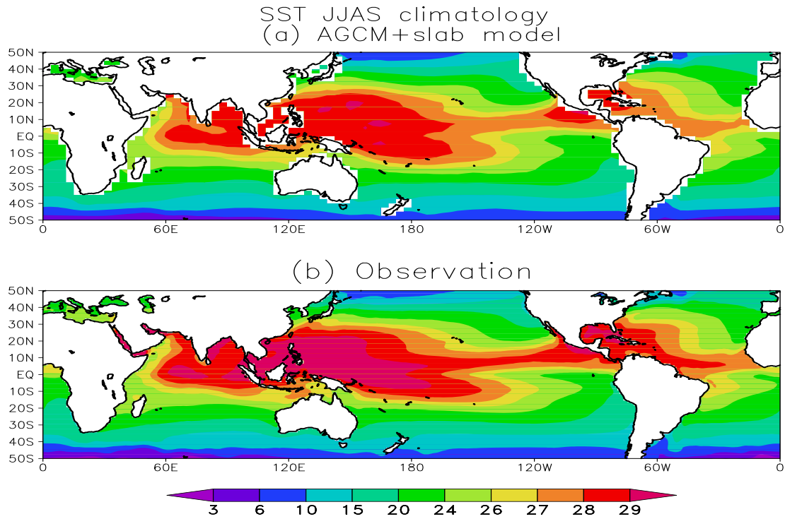
Figure 1: JJAS SST (°C) climatology based on 1984-2003 (a) AGCM+slab model (b) observation
