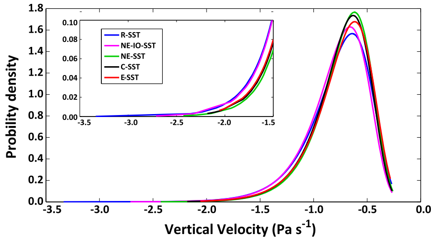
FIG. 4. Fitted Weibull PDF of minimum daily midtropospheric (500 hPa) vertical velocity (unit: \text{Pa s}^{-1} ) time series extracted from the northwest Pakistan region ( 30^{\circ} – 36^{\circ}\text{N} , 70^{\circ} – 74^{\circ}\text{E} ) during JJAS for the C-SST (black), R-SST (blue), E-SST (red), NE-SST (green), and NE-IO-SST (purple) sets of experiments. The inset shows the details of the left tail of the PDFs, which describes the occurrence of extreme daily events in the simulations. The x axis is 500-hPa vertical velocity, and upward vertical velocity is negative. The y axis is probability density.
