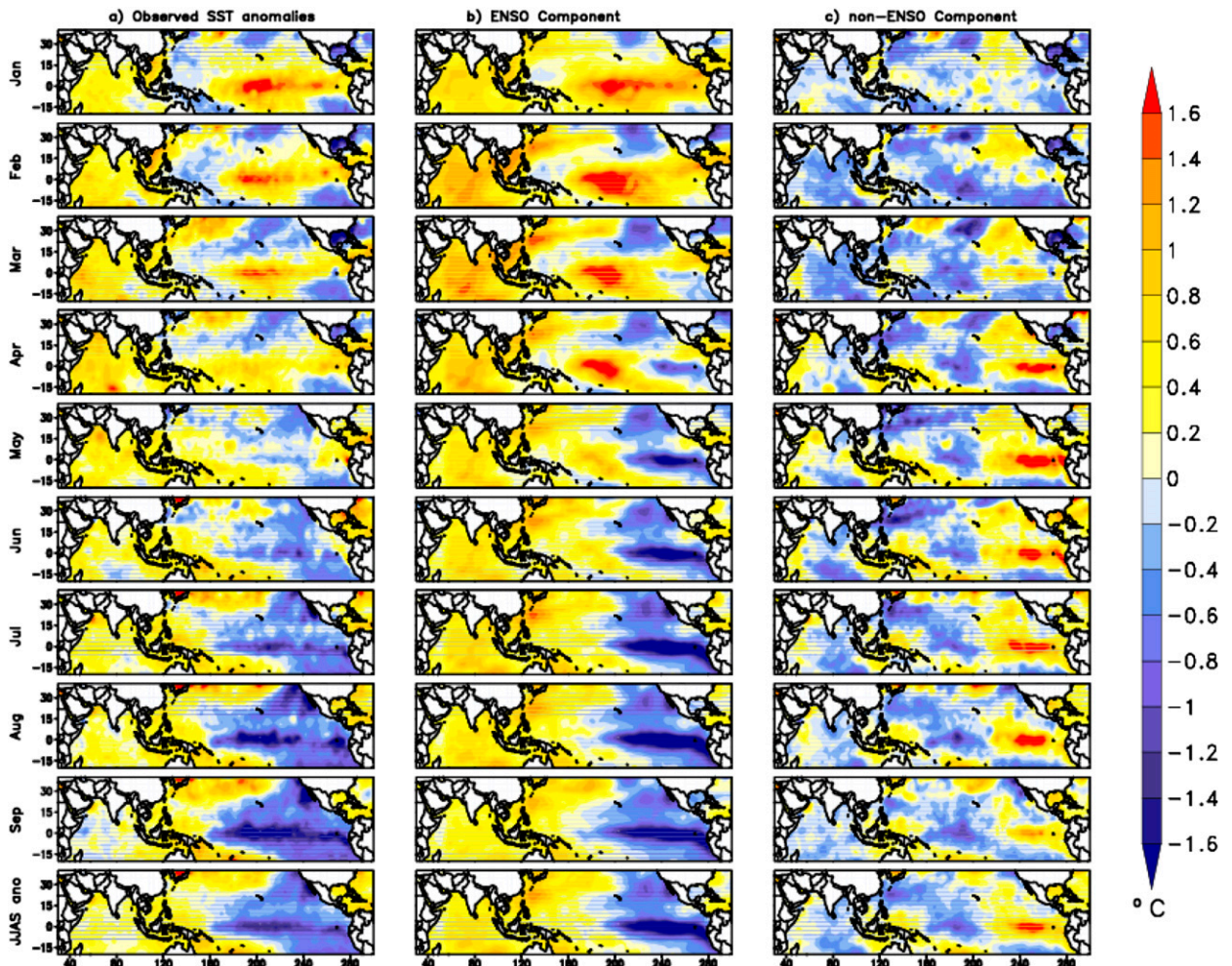
FIG. 1. January–September monthly evolution of SST anomalies ( ^{\circ}\text{C} ) and JJAS seasonal mean SST anomalies during 2010 for (a) observed SST anomalies, (b) ENSO component, and (c) ENSO-unrelated component. ENSO-related and ENSO-unrelated SST patterns were estimated from monthly SST anomalies during 2010 following Compo and Sardeshmukh (2010). SST anomalies are computed from the base period 1948–2010. Monthly SSTs are taken from HadISST (Rayner et al. 2003).
