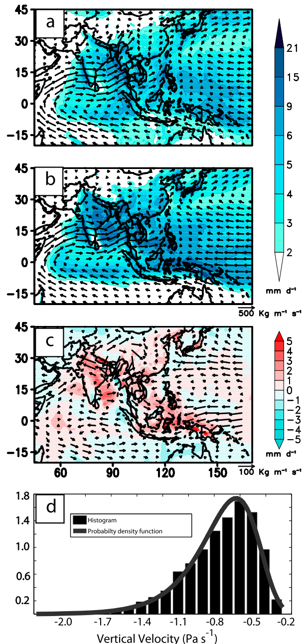
FIG. 2. Spatial distribution of mean rainfall (shaded; unit: \text{mm day}^{-1} ) superimposed on mean vertically integrated moisture transport vectors (unit: \text{Kg m}^{-1} \text{s}^{-1} ) for JJAS seasonal average for (a) TRMM rainfall climatology for the base period (1998–2010) and moisture transport NCEP climatology (1950–2010) and (b) ensemble mean of C-SST runs. The moisture transport vectors are integrated from the surface pressure to the 300-hPa level. (c) Differences of rainfall and moisture transport between C-SST simulated and TRMM and NCEP climatologies. (d) Histogram (black bars) of minimum daily mid-tropospheric (500 hPa) vertical velocity time series extracted from the northwest Pakistan region ( 30^{\circ} – 36^{\circ}\text{N} , 70^{\circ} – 74^{\circ}\text{E} ) during JJAS in the C-SST experiments with fitted Weibull PDF (black curve). The x axis is 500-hPa vertical velocity (unit: \text{Pa s}^{-1} ), and upward vertical velocity is negative. The y axis is probability density. The histogram is normalized by area (e.g., bin width by number of observations in each bin) for better comparison with the fitted PDF. See text for further details.
