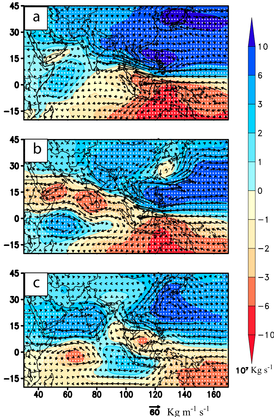
FIG. 9. JJAS anomalies of streamfunction (unit: 10^7 \text{ Kg s}^{-1} ) and rotational component of vertically integrated water vapor transport vector ( \text{Kg m}^{-1} \text{ s}^{-1} ) for (a) R-SST runs, (b) E-SST runs, and (c) NE-SST runs. Anomalies significant at the 95% confidence level (using a Student two-tailed test) are dotted.
