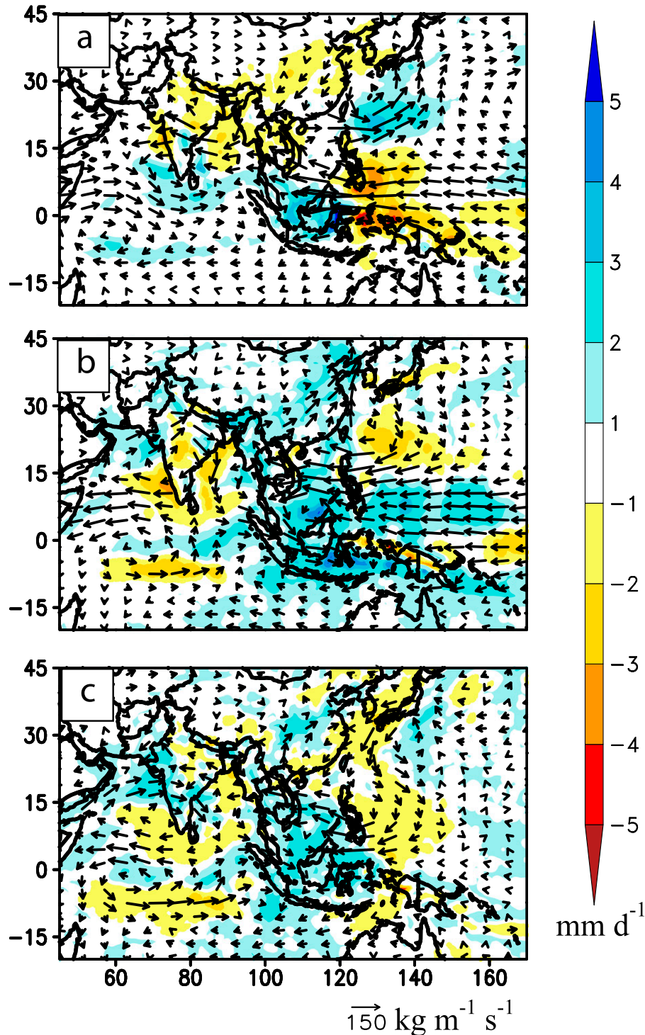
FIG. 6. As in Fig. 3, but for rainfall and vertically integrated moisture transport anomalies during JJAS 2010 in (a) E-SST runs, (b) NE-SST runs, (c) NE-IO-SST runs.
