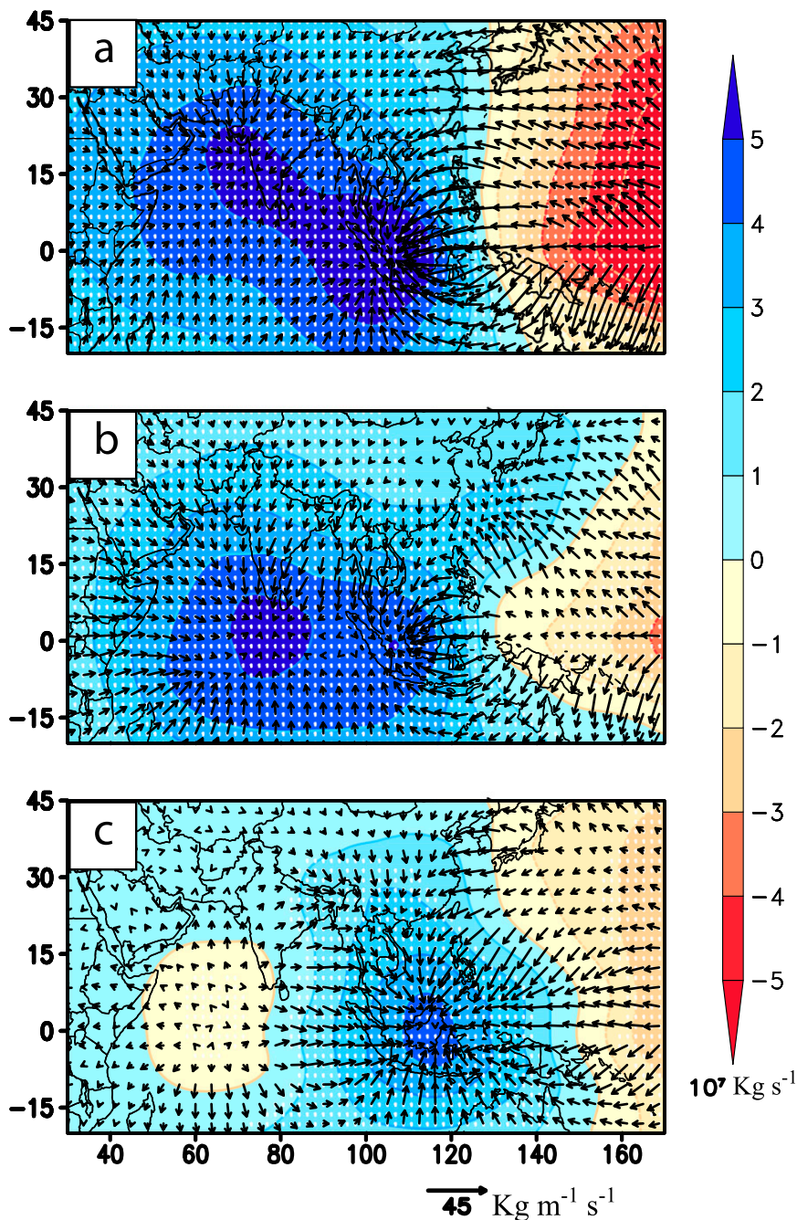
FIG. 7. JJAS anomalies of potential function (unit: 10^7 \text{ Kg s}^{-1} ) and divergent component of vertically integrated water vapor transport vector ( \text{Kg m}^{-1} \text{ s}^{-1} ) for (a) R-SST runs, (b) E-SST runs, and (c) NE-SST runs. Water vapor transport vectors are vertically integrated from the surface to 300 hPa. The potential function and divergent component of vertically integrated water vapor transport vectors are estimated on a global domain but are shown here only over the region of interest (Chen 1985; Krishnan 1998). The anomalies are computed from the JJAS climatology of potential function and divergent component of vertically integrated water vapor transport in the C-SST runs. Anomalies significant at the 95% confidence level (using a Student two-tailed test) are dotted.
