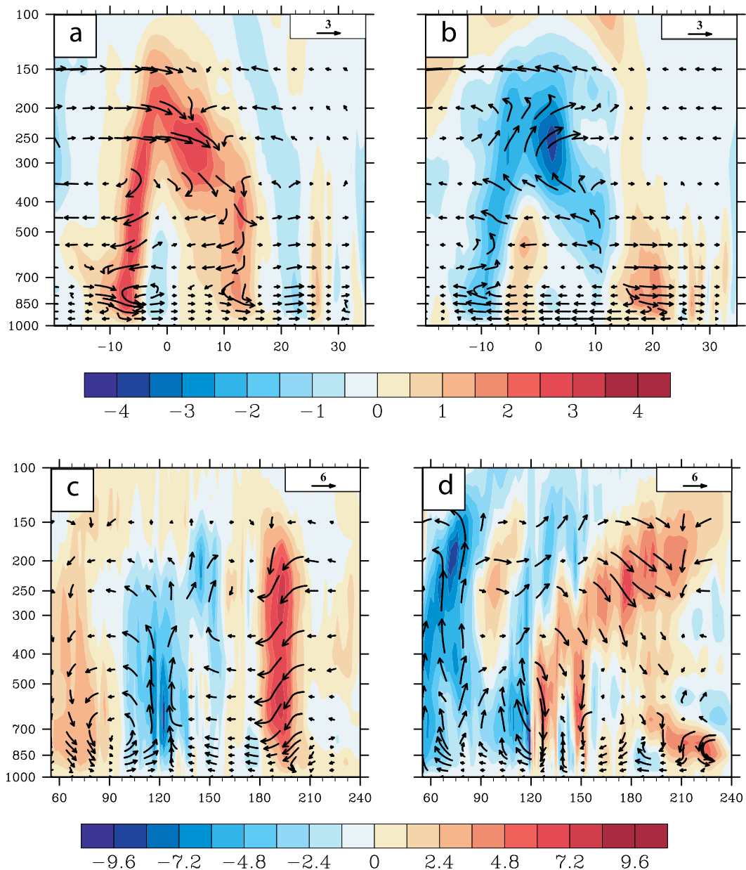
FIG. 8. (a) North–south cross section of zonally averaged ( 60^{\circ} – 75^{\circ} E) meridional and vertical wind anomalies over the west Indian Ocean (domain: 20^{\circ} S– 35^{\circ} N) during JJAS of 2010 for NE-SST runs. (b) As in (a), but for E-SST runs. (c) East–west cross section of meridionally averaged ( 15^{\circ} S– 0^{\circ} ) zonal and vertical wind anomalies for the domain 30^{\circ} – 240^{\circ} E during JJAS of 2010 for NE-SST runs. (d) As in (c), but for E-SST runs. Upward vertical velocity is negative in all panels. The wind anomalies for the NE-SST and E-SST runs are relative to the climatology estimated from the C-SST runs.
