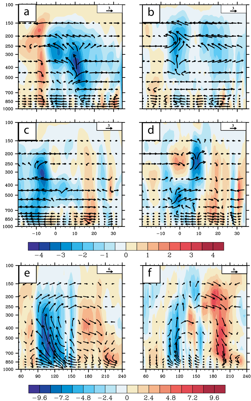
FIG. 5. (a) North–south cross section of zonally averaged ( 60^{\circ} – 75^{\circ} E) meridional and vertical wind anomalies over the west Indian Ocean (domain: 20^{\circ} S– 35^{\circ} N) during JJAS of 2010 from NCEP. (b) As in (a), but for R-SST runs. (c) North–south cross section of zonally averaged ( 85^{\circ} – 110^{\circ} E) meridional and vertical wind anomalies over the east Indian Ocean (domain: 20^{\circ} S– 40^{\circ} N) during JJAS of 2010 from NCEP. (d) As in (c), but for R-SST runs. (e) East–west cross section of meridionally averaged ( 15^{\circ} S– 0^{\circ} ) zonal and vertical wind anomalies for the domain 30^{\circ} – 240^{\circ} E during JJAS of 2010 from NCEP. (f) As in (e), but for R-SST runs. Upward vertical velocity is negative in all panels. The wind anomalies for the R-SST runs are relative to the climatology estimated from the C-SST runs. NCEP wind anomalies are computed from the 1950–2010 climatology. East–west circulation is plotted after removing the zonal mean from the circulation parameters.
