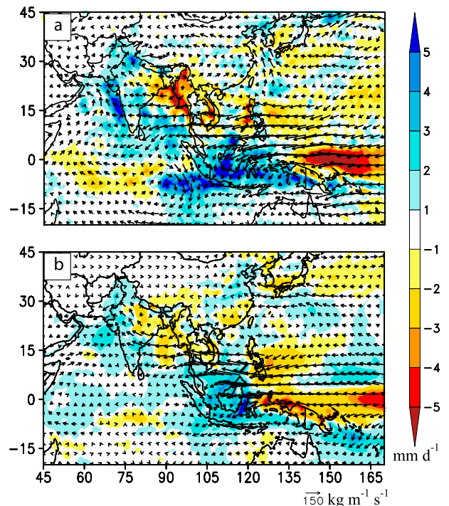
FIG. 3. Rainfall (shaded; unit: \text{mm day}^{-1} ) and vertically integrated moisture transport (unit: \text{Kg m}^{-1} \text{s}^{-1} ) anomalies during boreal summer of 2010 for (a) TRMM rainfall (shaded) and NCEP moisture transport (vector) and (b) R-SST runs. For observations, rainfall (vertically integrated moisture transport) anomalies are computed from the base period 1998–2010 (1950–2010). The R-SST rainfall and vertically integrated moisture transport anomalies are relative to the climatology estimated from the C-SST runs.
