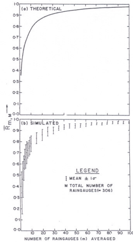
Figure 2. Increase in the correlation coefficient between mean series of m selected gauges and the all-India rainfall series ( \bar{R}_{m,M} ) with the increase in m . (a) Theoretical curve derived from equation (2), and (b) simulated curve with actual data
