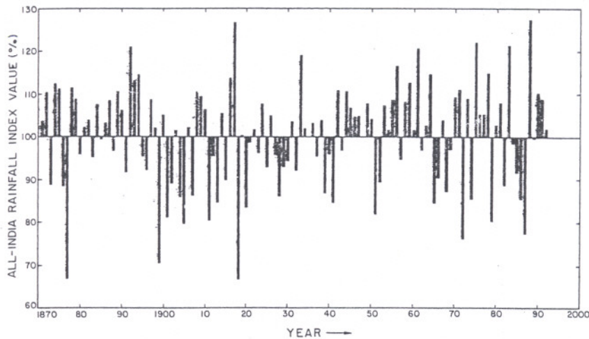
Figure 5. A reconstructed all-India summer monsoon rainfall series for the period 1871–1992
