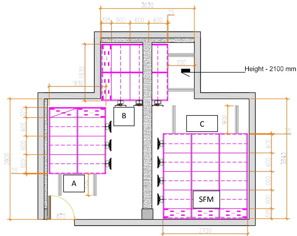
PLAN OF LAYOUT OF COMPACTORS
