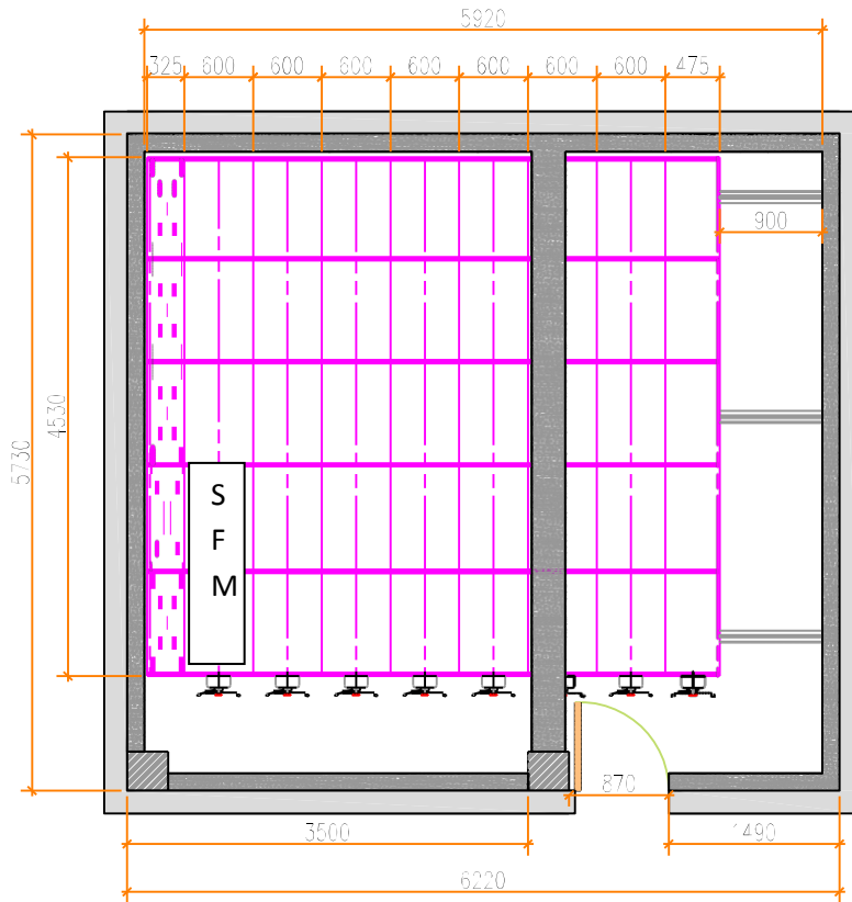
PLAN OF LAYOUT OF COMPACTORS
